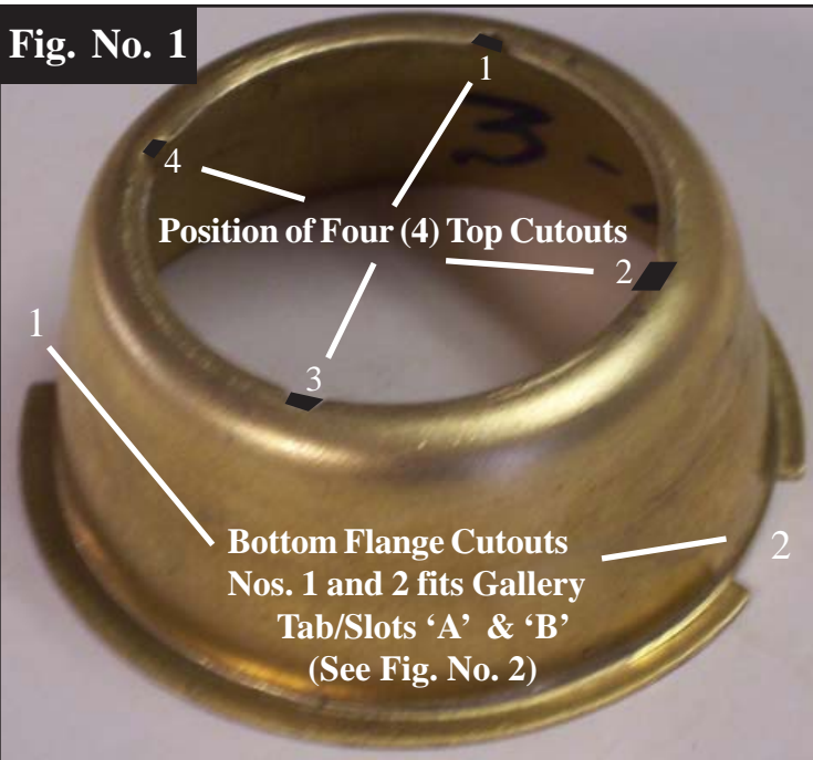
N146A Kone Kap Mantle Adaptor (Enlarged View)
